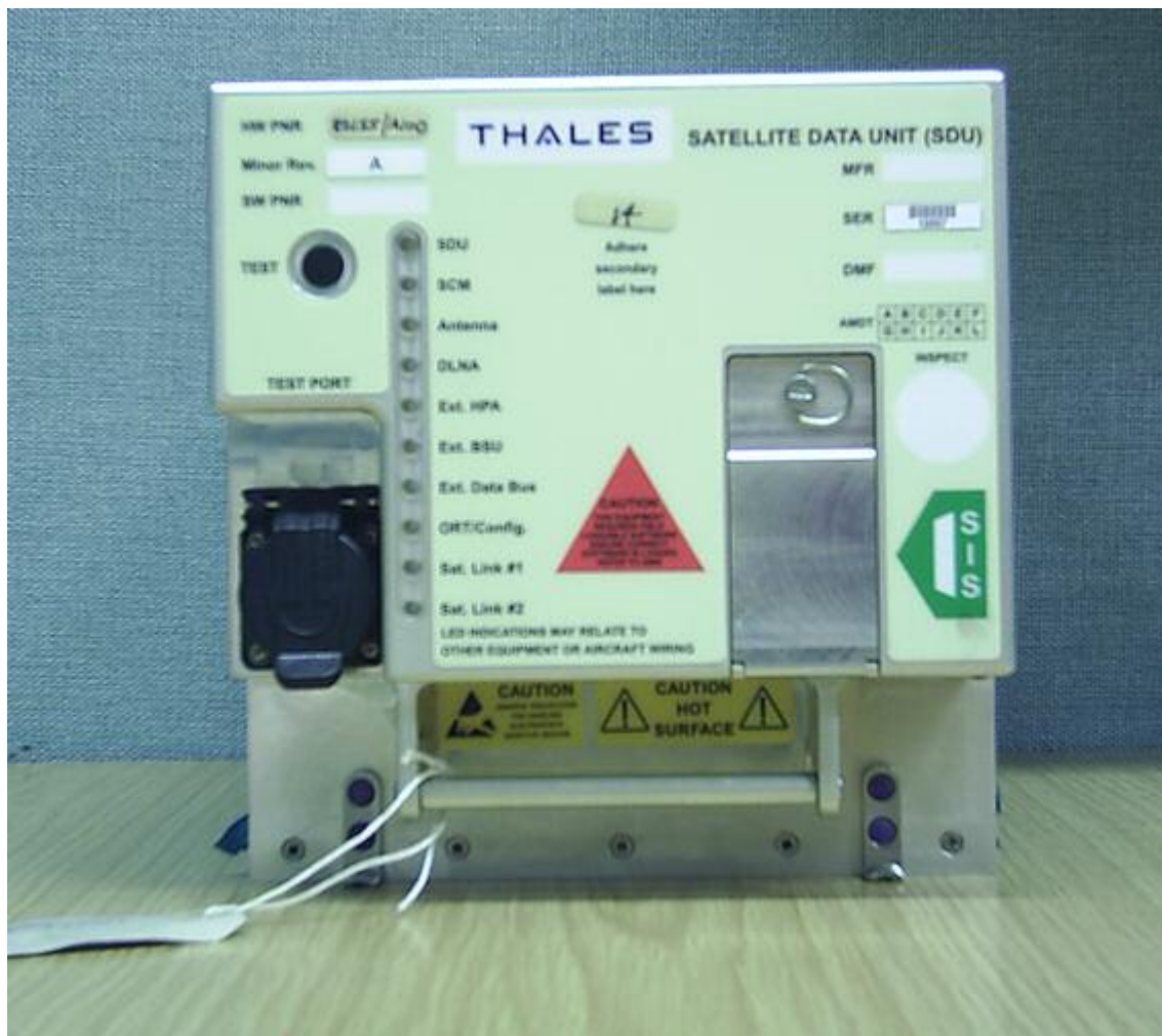
Figure 3: SDU Front
