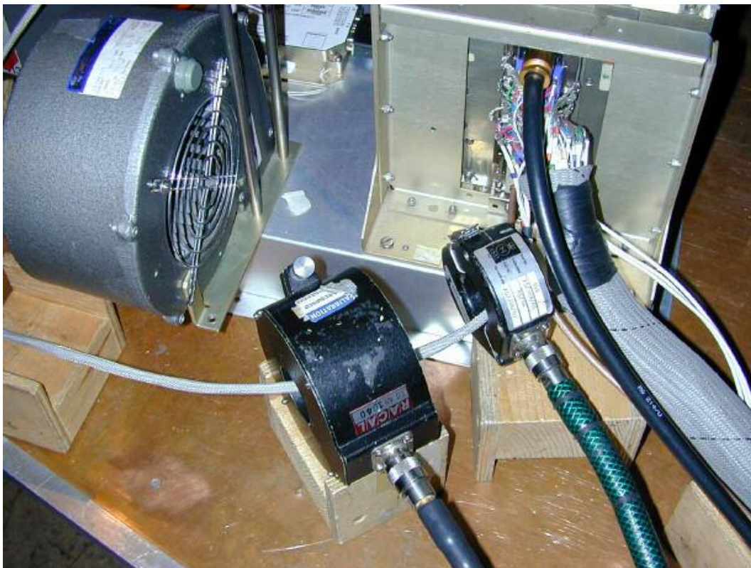
Figure 6: Conducted Susceptibility
