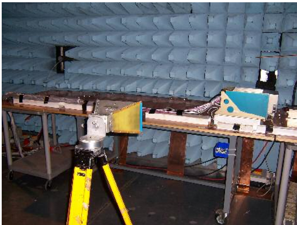
Figure 1: DO-160E (modified) Radiated Emissions
