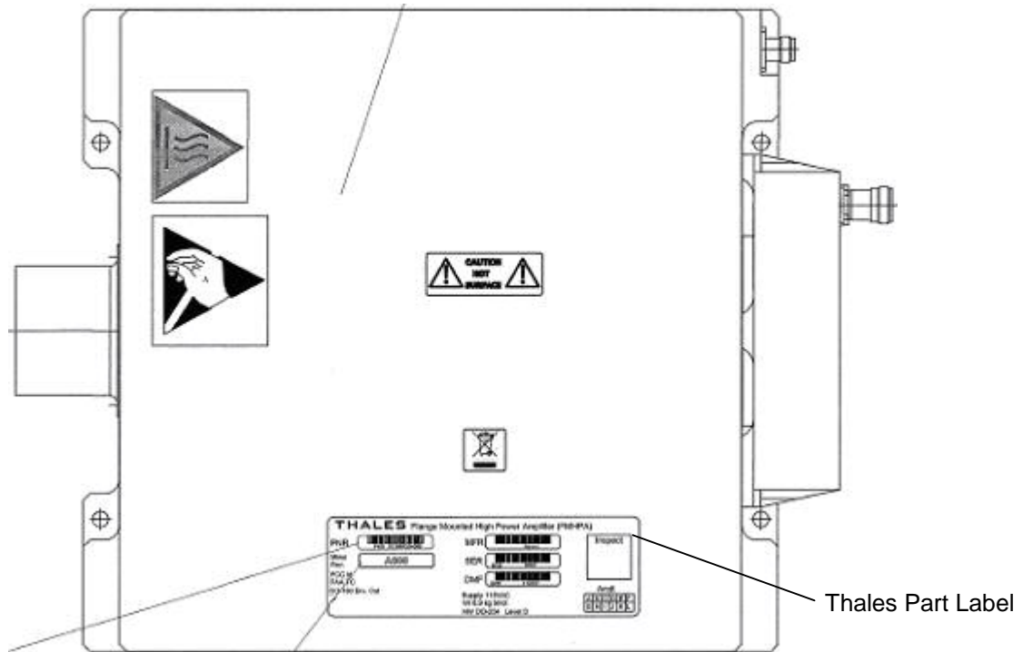
Figure 1: Placement of Part Label on FMHPA top panel
