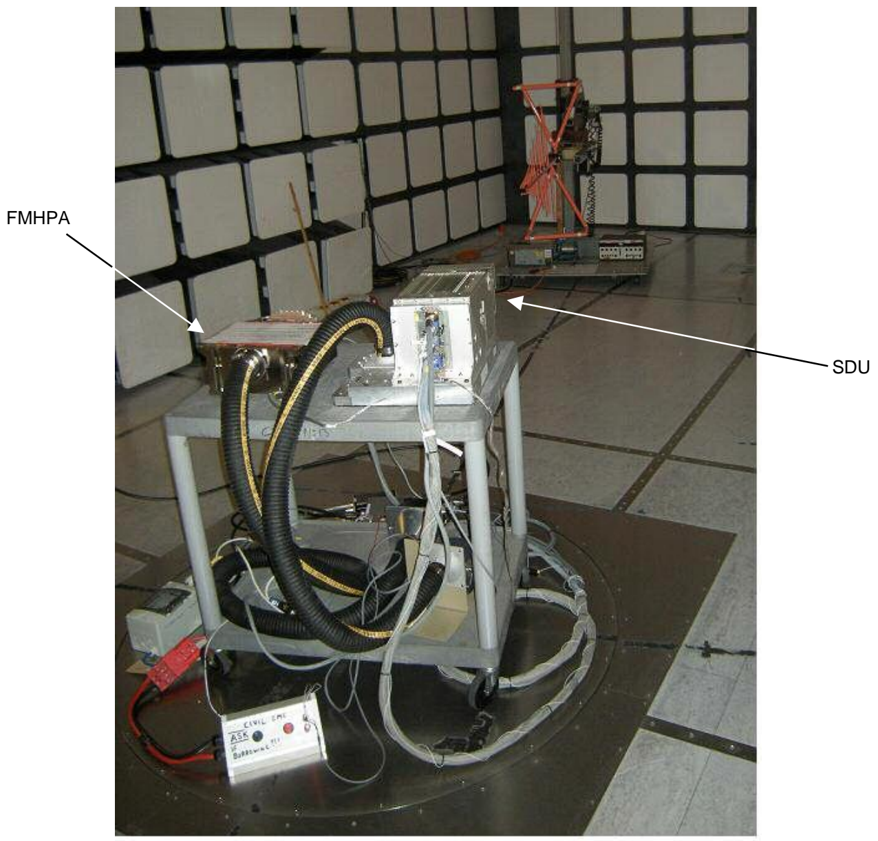
Radiated Emissions – 30 MHz to 1 GHz
