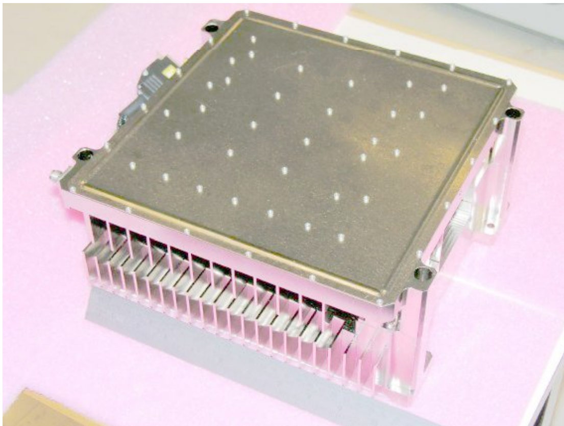
Figure 1: FMHPA assembled, top/front/right
