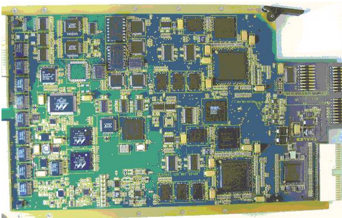
Figure 2: SDU Communication Processor Module (CPM) Top
