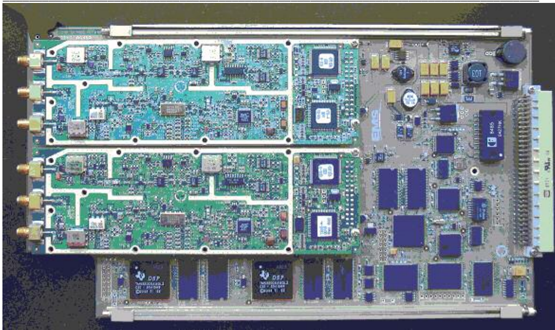
Figure 3: SDU Channel Card Module (CCM) Top
