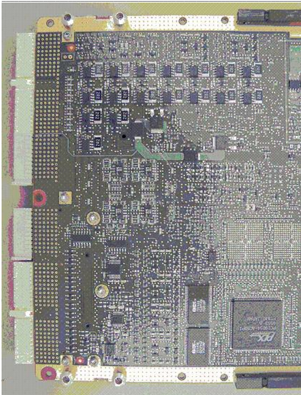
Figure 2: SDU Avionics Processor Module (APM) Bottom. Enlarged view of Left Side of Board.
