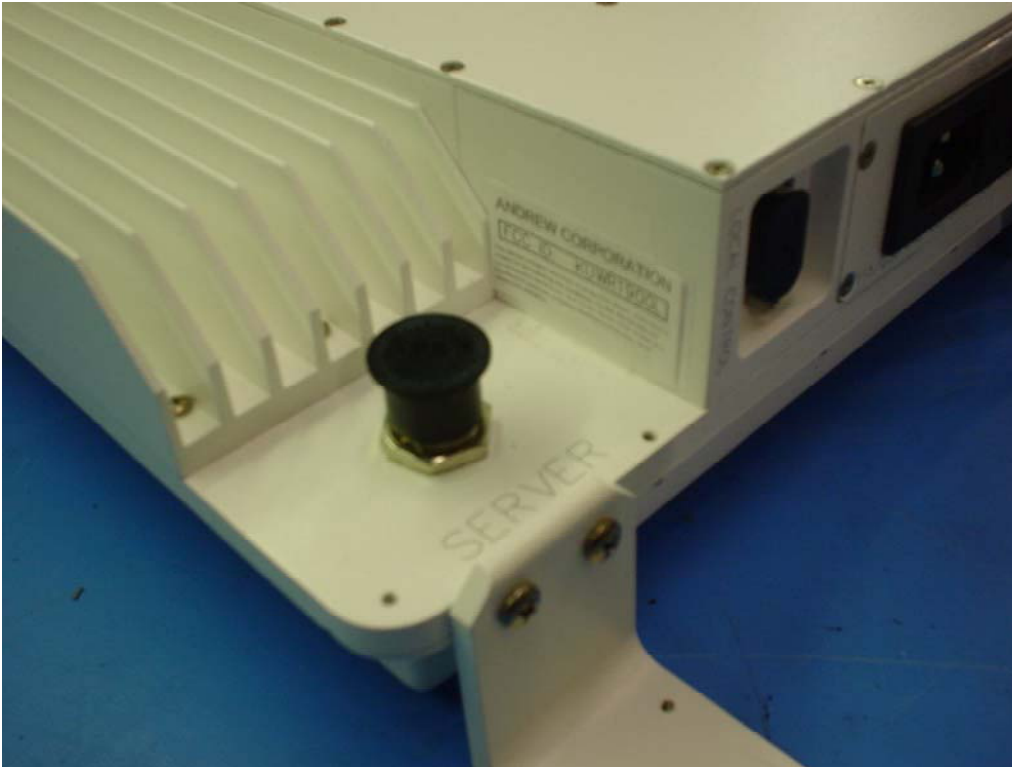
Figure 6. Location of FCCID Tag for KUWR1900L/KUWR800L
