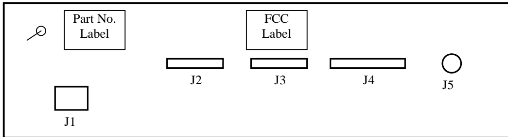
Figure 2 BDR (385700-3000) FCC Label Location
