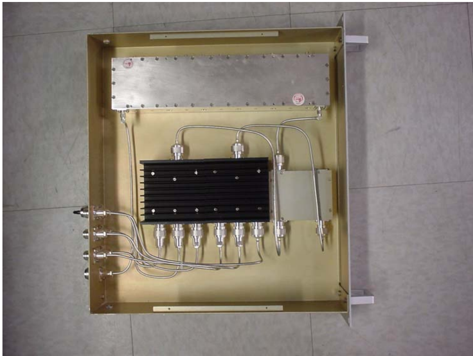
VHF Combiner
