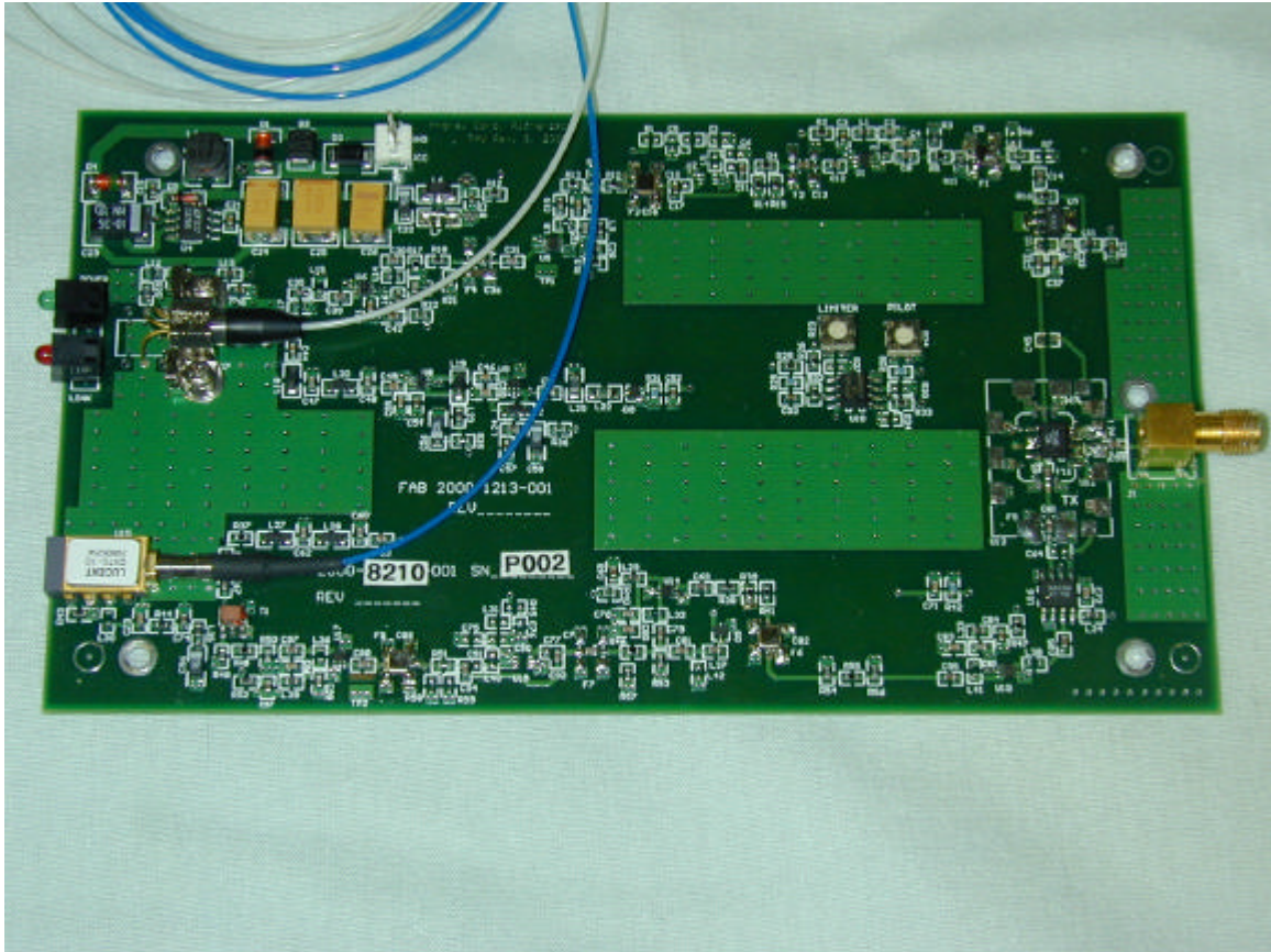
Photo 1 - RAU board, component side
