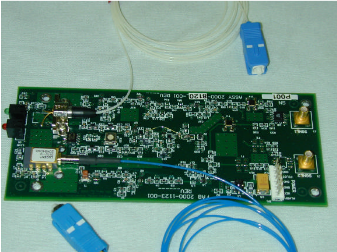
Photo 5 - CDU, RF board component side
