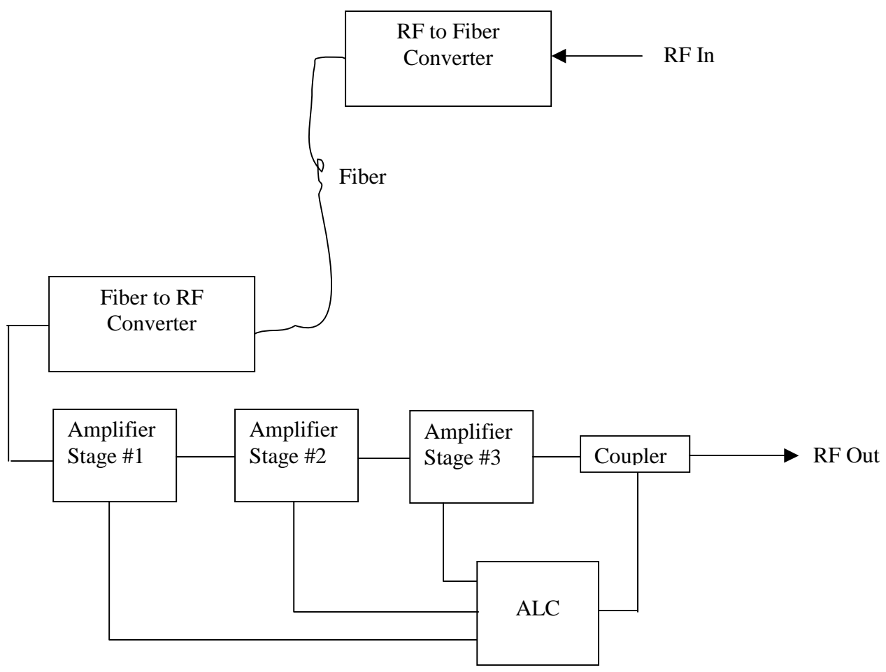
Downlink Block Diagram
