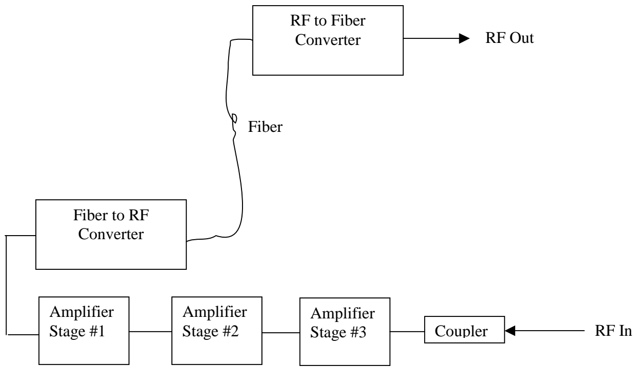
Uplink Block Diagram
