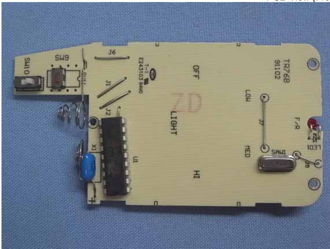
Photo 4 PCB View (Front Side)
