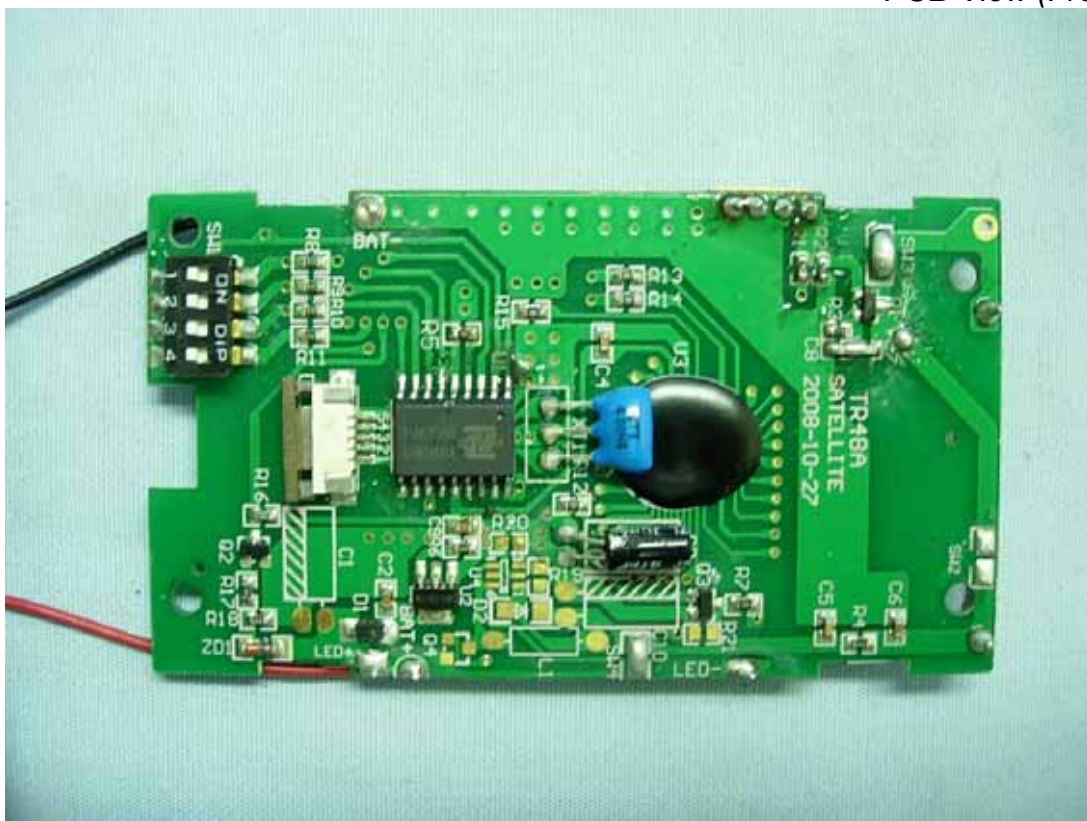
Photo 5 PCB View (Front Side)
