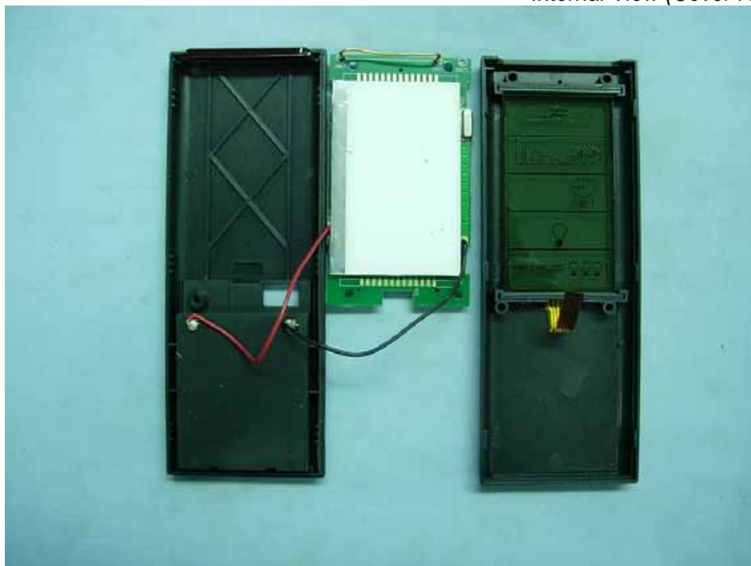
Photo 3 Internal View (Cover Removed)
