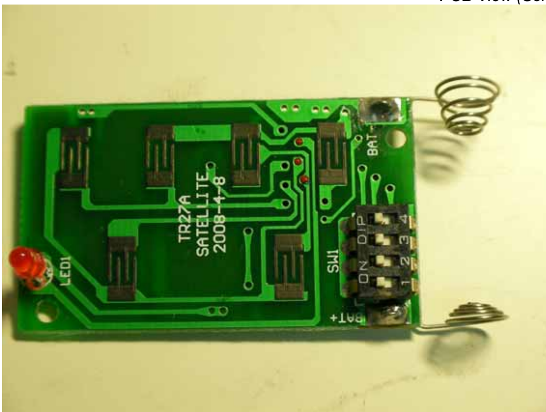
Photo 6 PCB View (Solder Side)
