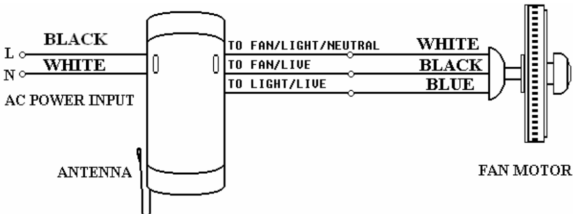
Ceiling Fan Remote Control Wiring Connection
