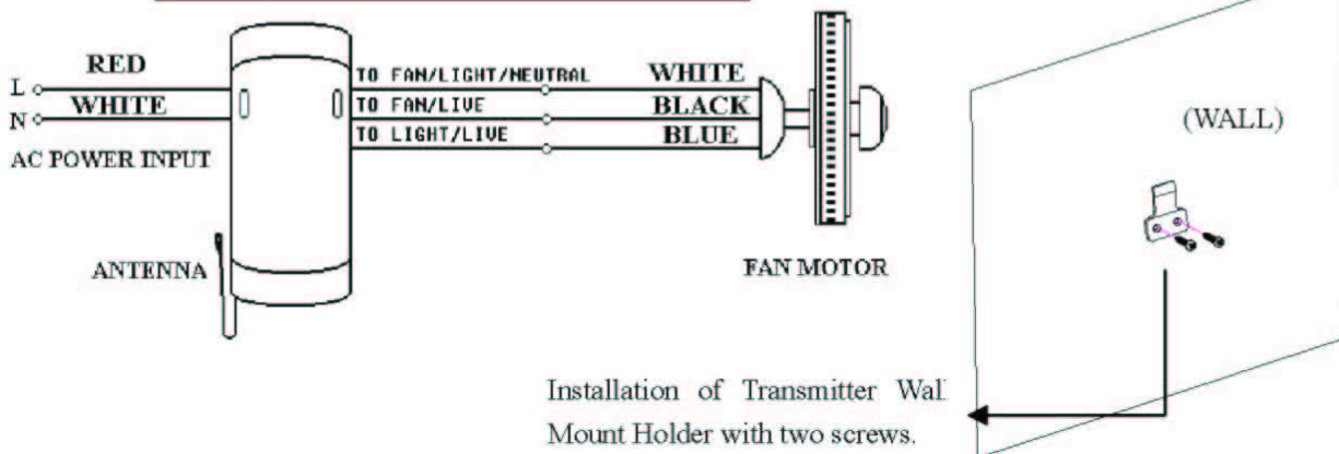
Ceiling Fan Remote Control Wiring Connection
