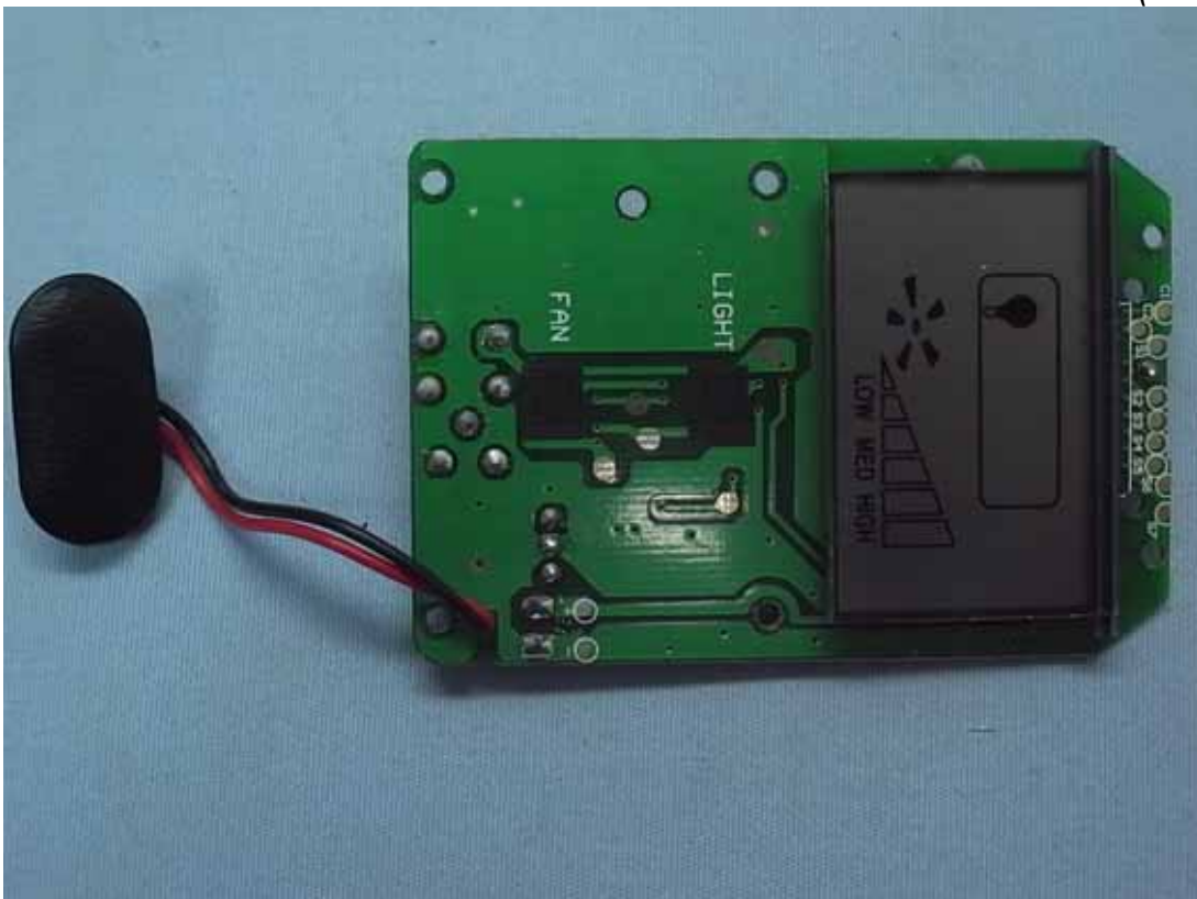
Photo 4 PCB View (Front Side)
