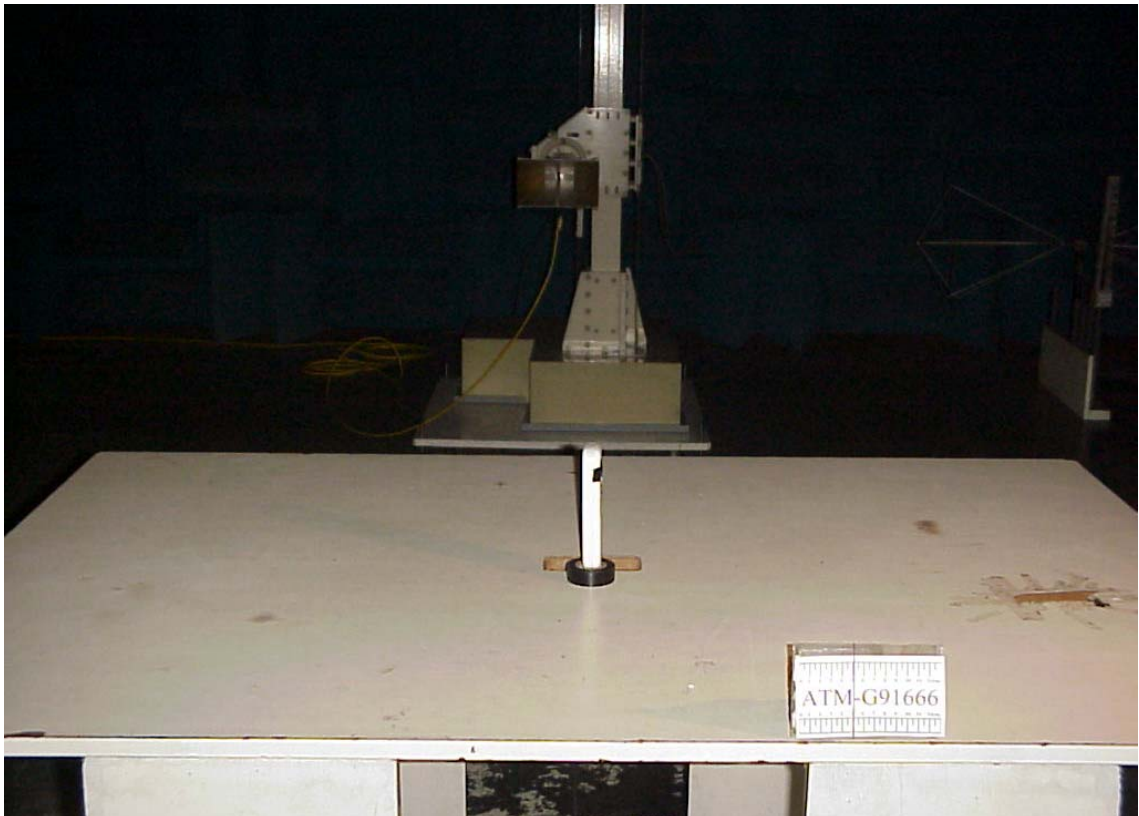
7.2. Photos of Radiated Measurement at Semi-Anechoic Chamber (1~3GHz) EUT on Stand
