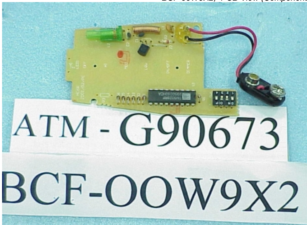
Photos 6 BCF-00W9X2, PCB View (Component Side)
