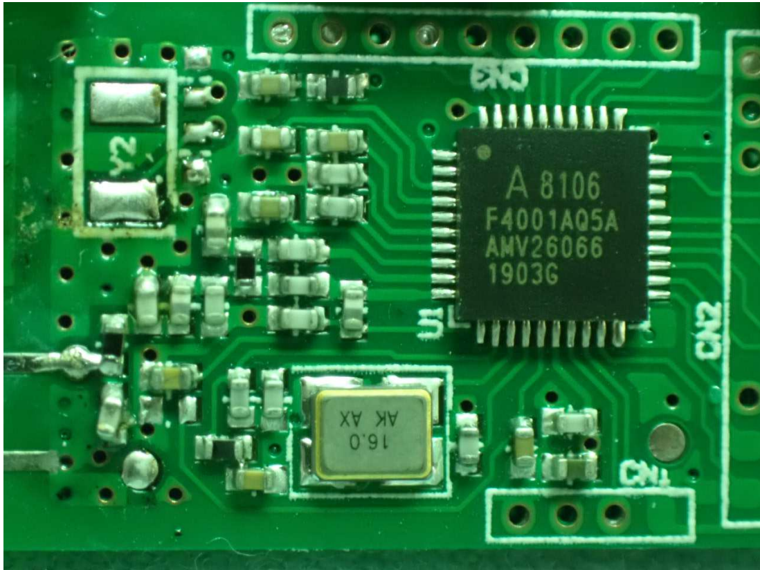
Figure 7 Internal View (RF Chip)
