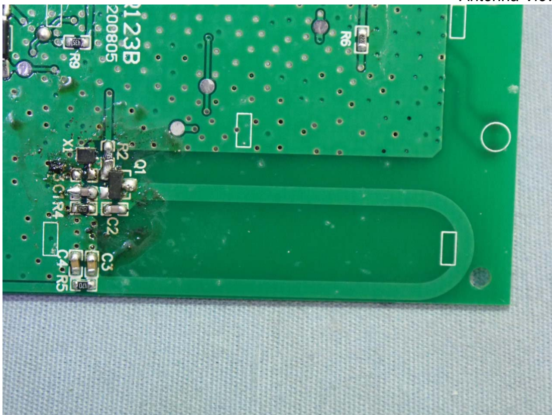
Figure 12 Antenna View
