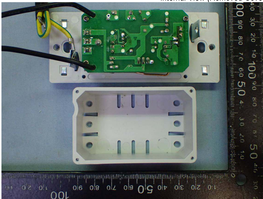
Figure 8 Internal View (Removed Cover)
