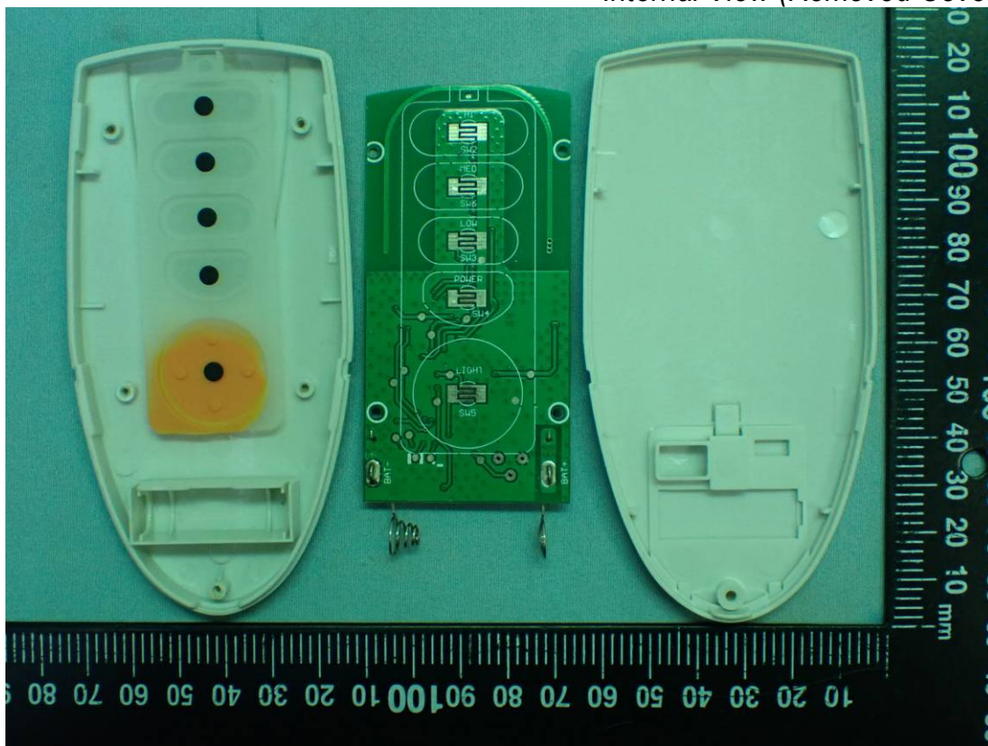
Figure 9 Internal View (Removed Cover)
