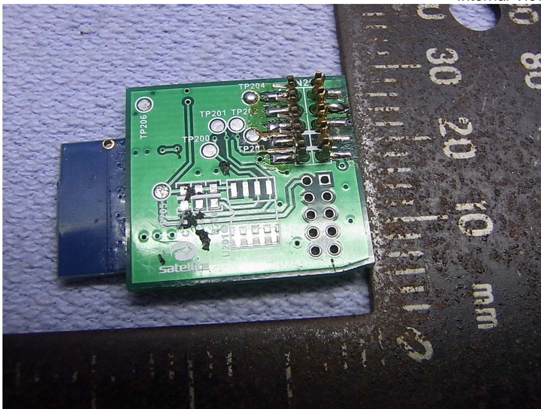
Figure 11 Internal View
