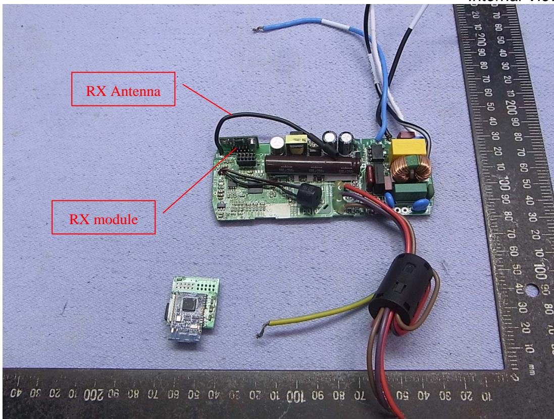
Figure 4 Internal View
