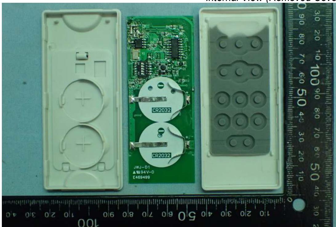
Figure 4 Internal View (Removed Cover)
