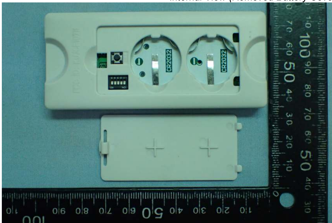
Figure 3 Internal View (Removed Battery Cover)
