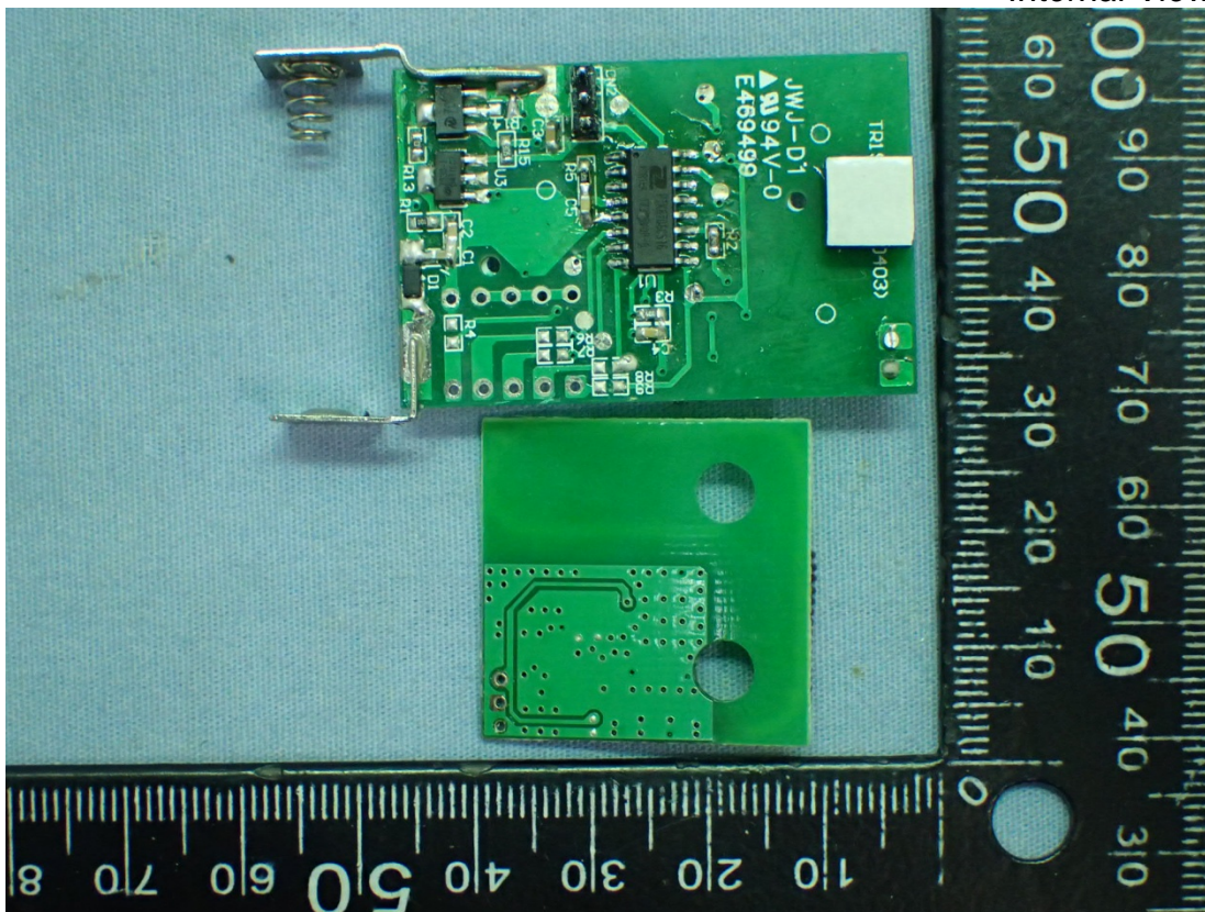
Figure 10 Internal View
