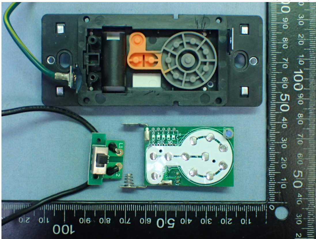
Figure 9 Internal View
