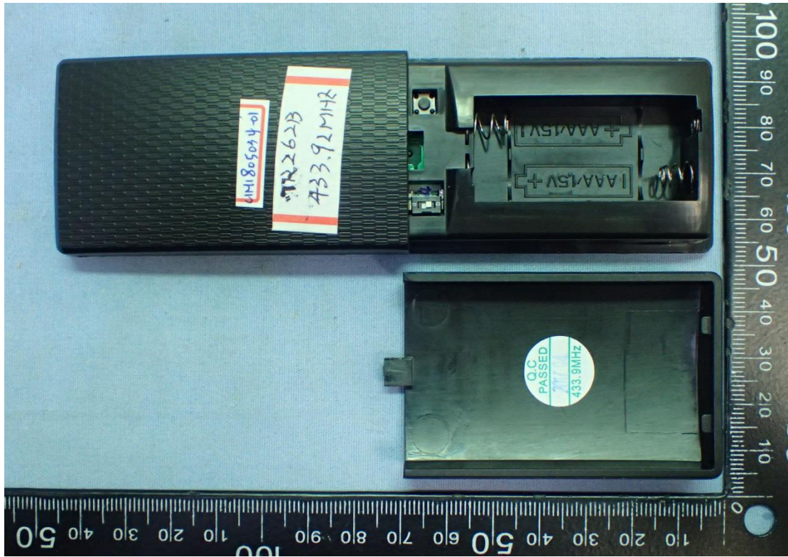
Figure 3 Internal View (Removed Battery Cover)
