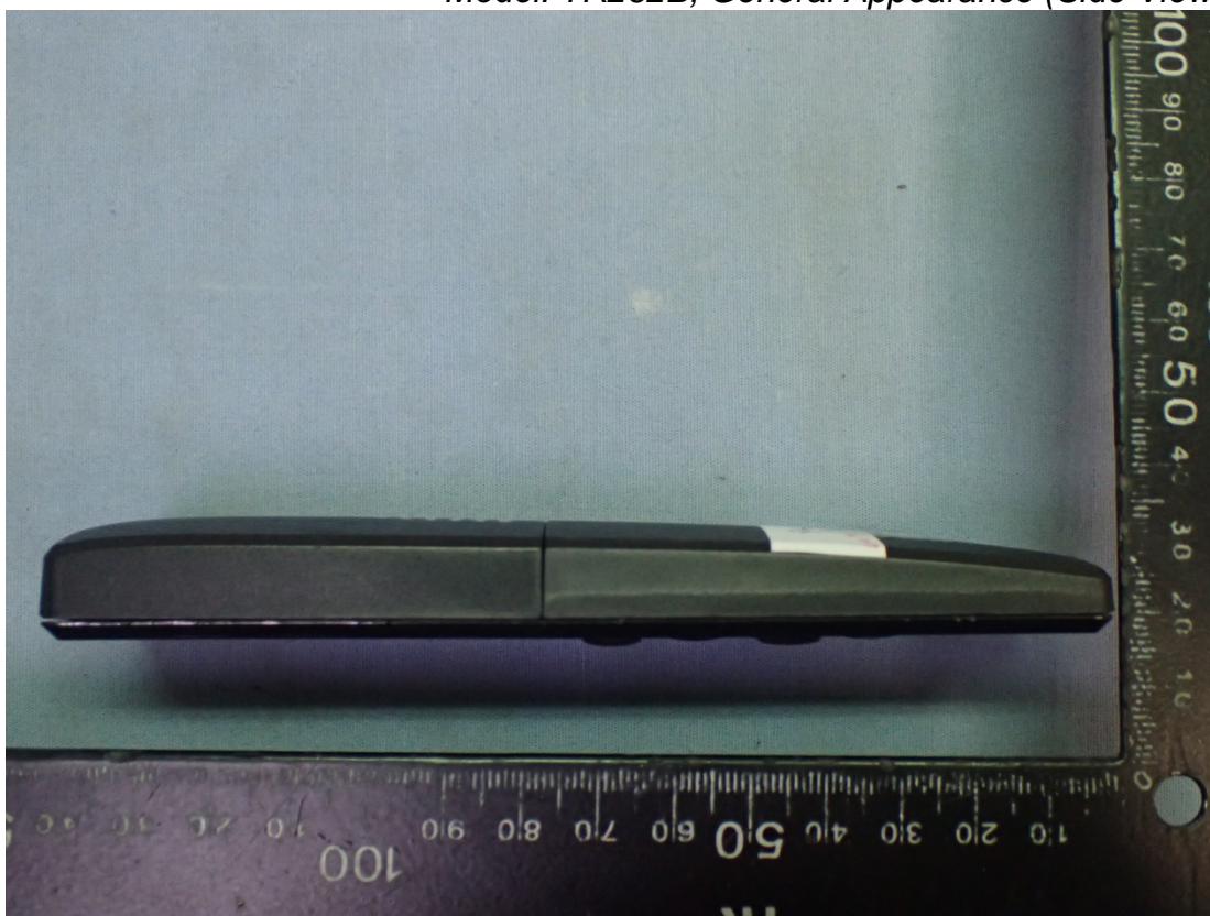
Figure 4 Model: TR262B, General Appearance (Side View)
