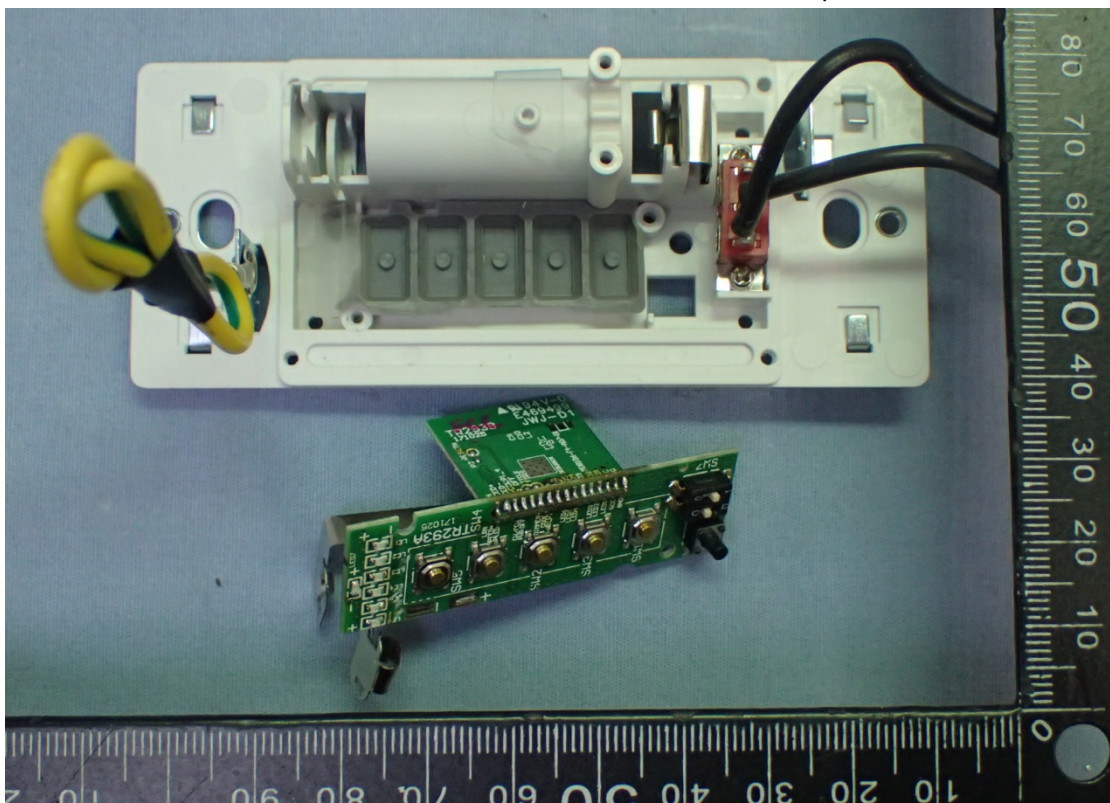
Figure 4 Internal View (Removed Control Boards)
