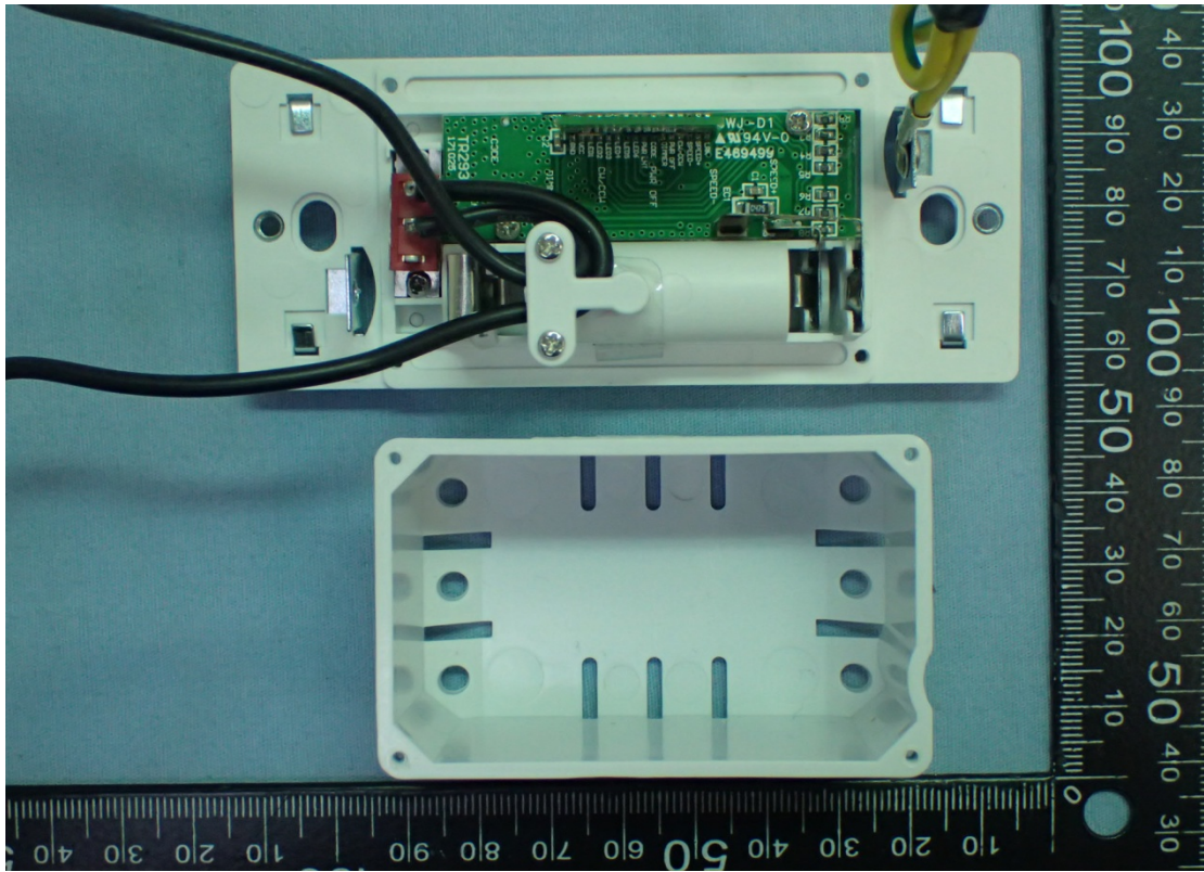
Figure 3 Internal View (Removed Cover)
