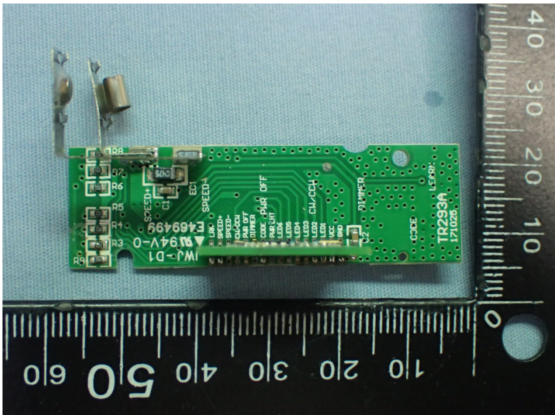
Figure 6 Internal View (Function Control Board, Back View)
