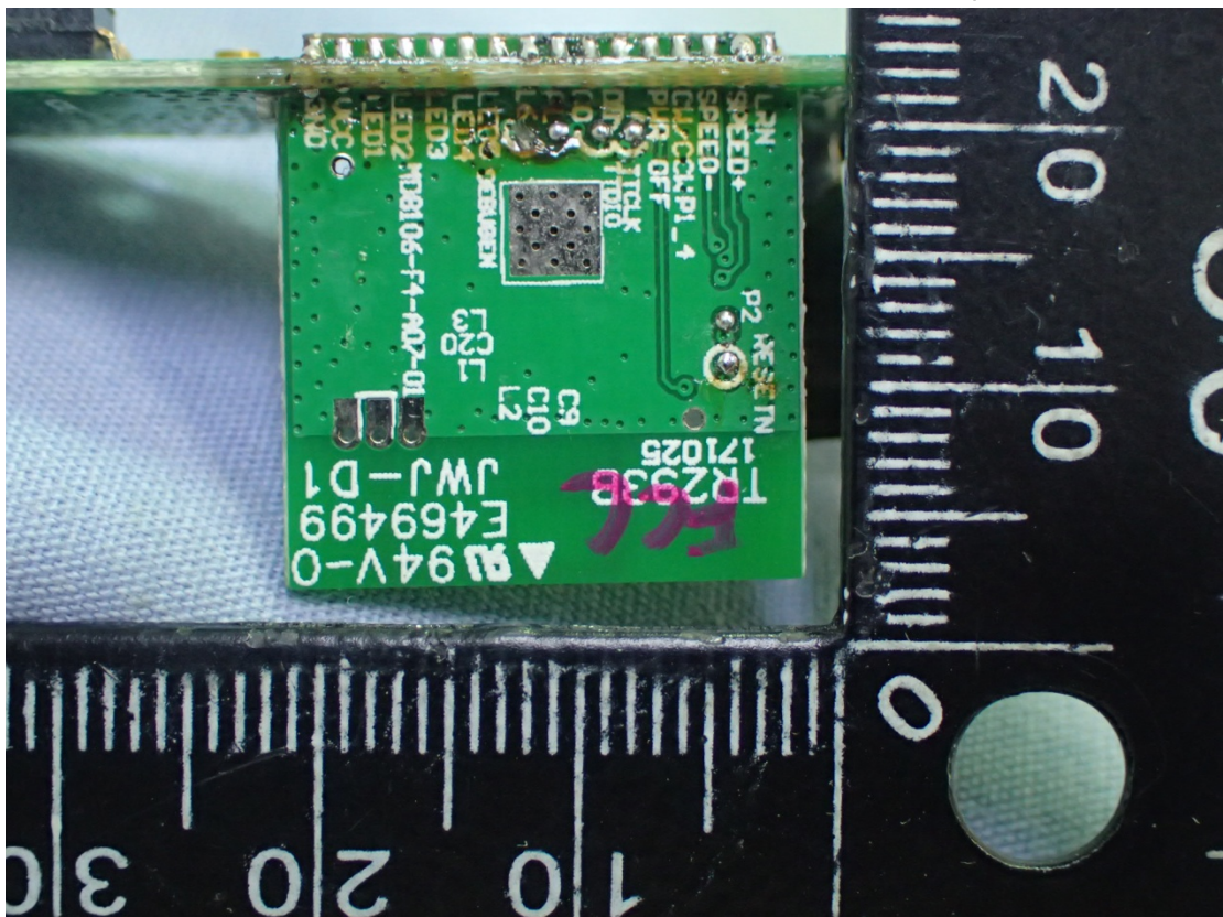
Figure 8 Internal View (RF Board, Back View)
