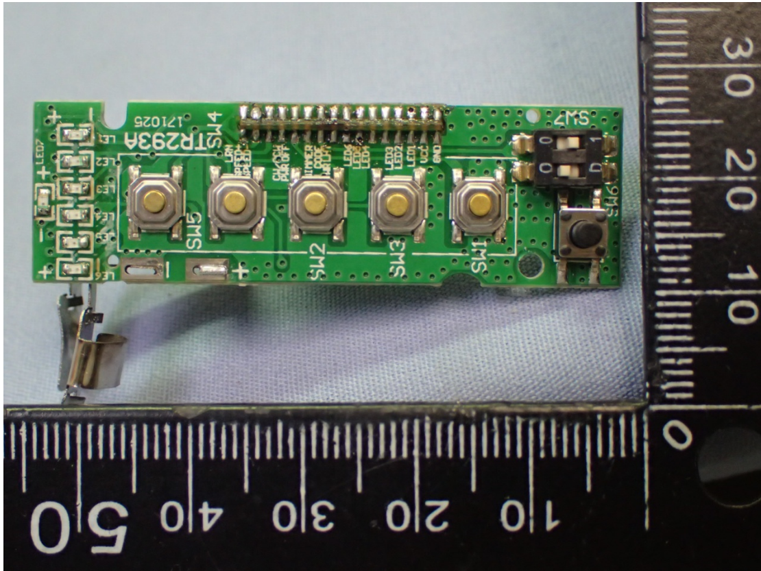
Figure 5 Internal View (Function Control Board, Front View)
