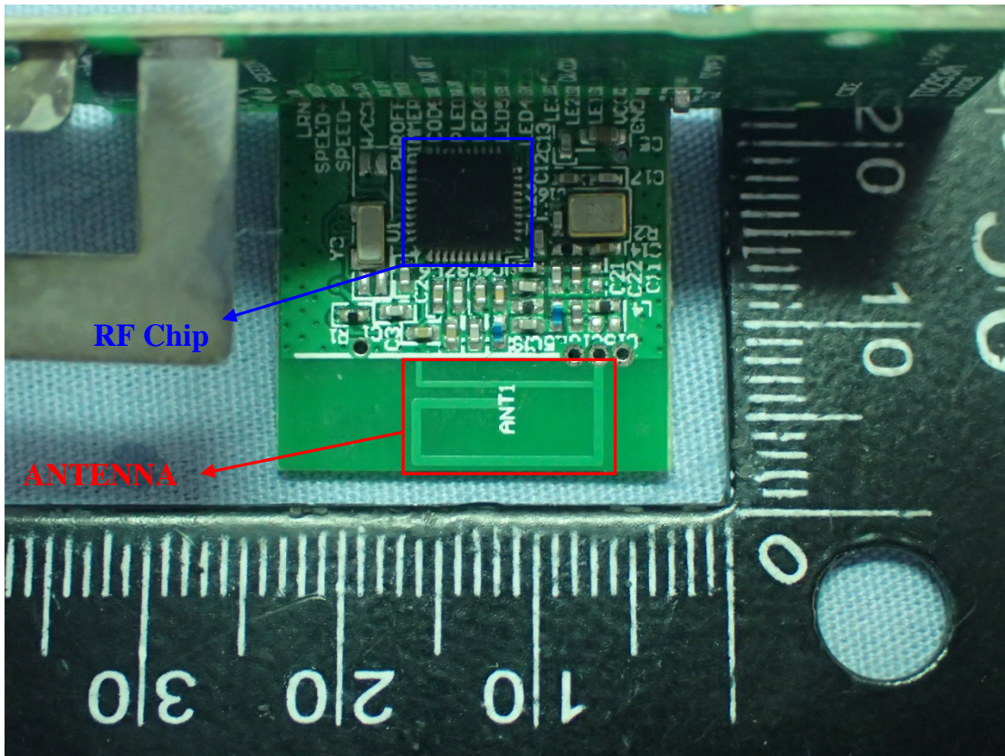
Figure 7 Internal View (RF Board, Front View)
