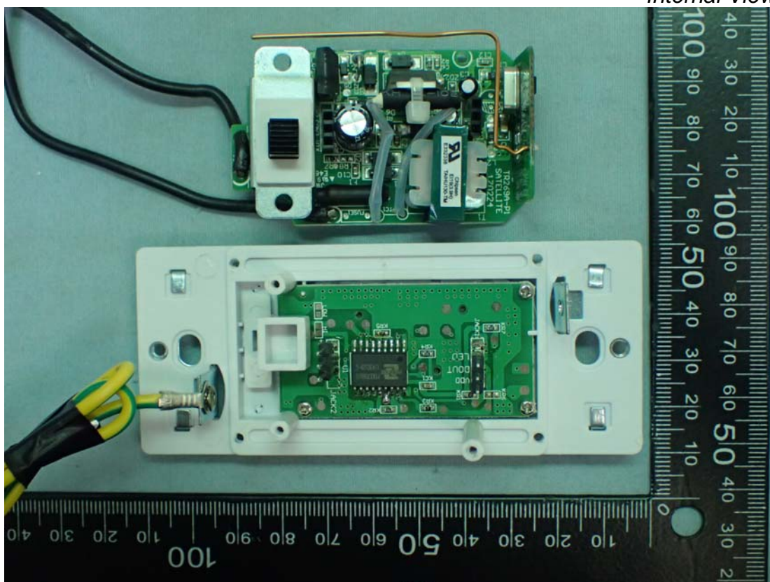
Figure 7 Internal View
