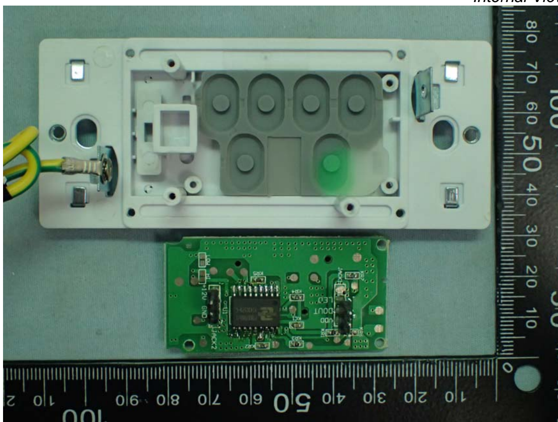
Figure 8 Internal View
