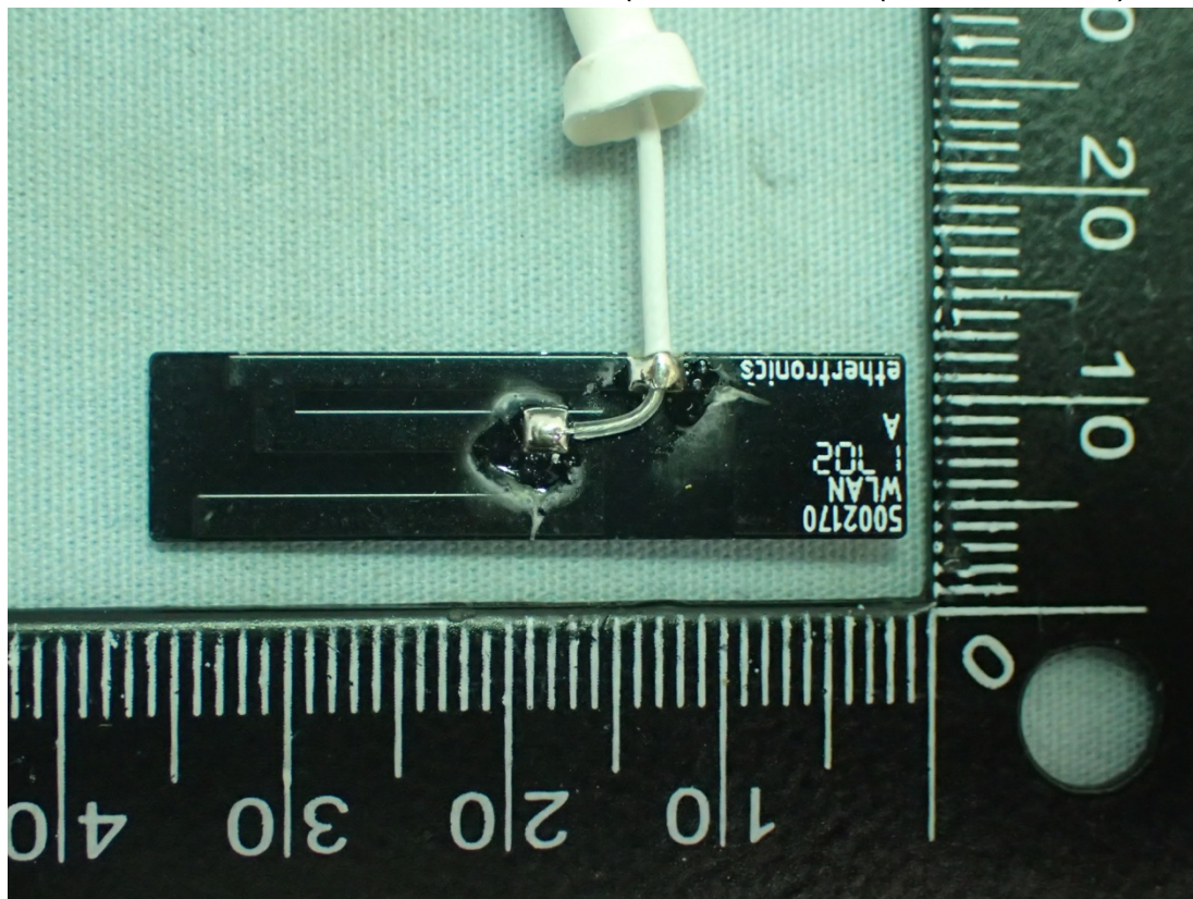
Figure 15 Internal View (WIFI Antenna (P/N: 5002170), Back View)
