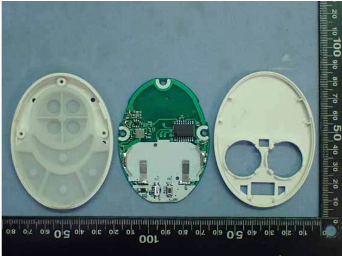
Photo 8 Internal View
