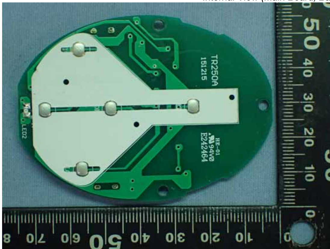
Photo 10 Internal View (Main Board, Back View)
