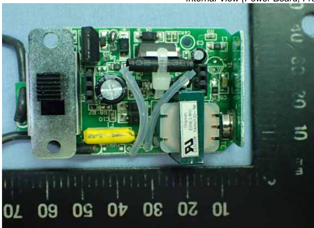
Photo 6 Internal View (Power Board, Front View)
