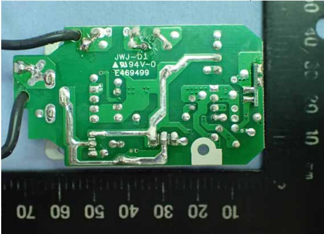
Photo 7 Internal View (Power Board, Back View)
