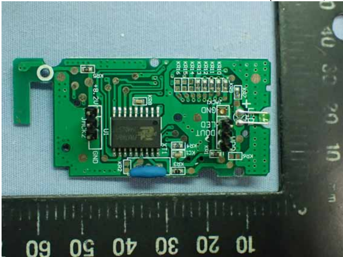
Photo 11 Internal View (Main Board, Front View)
