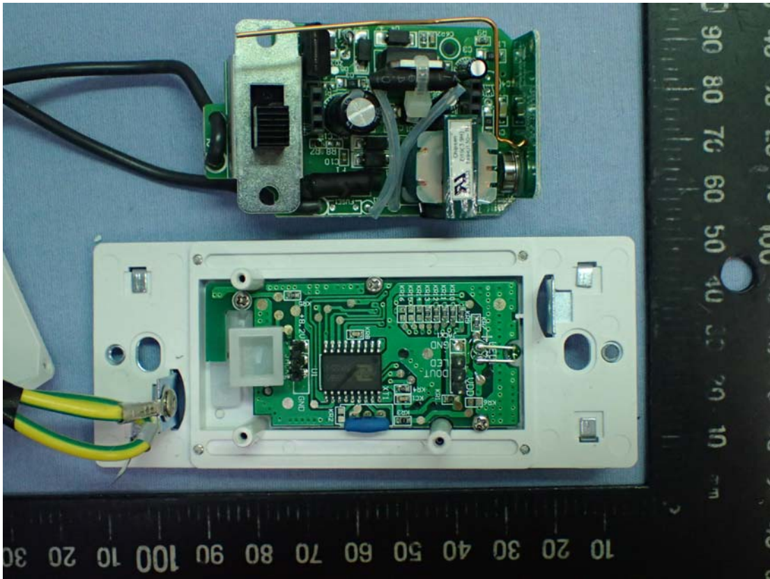
Photo 6 Internal View
