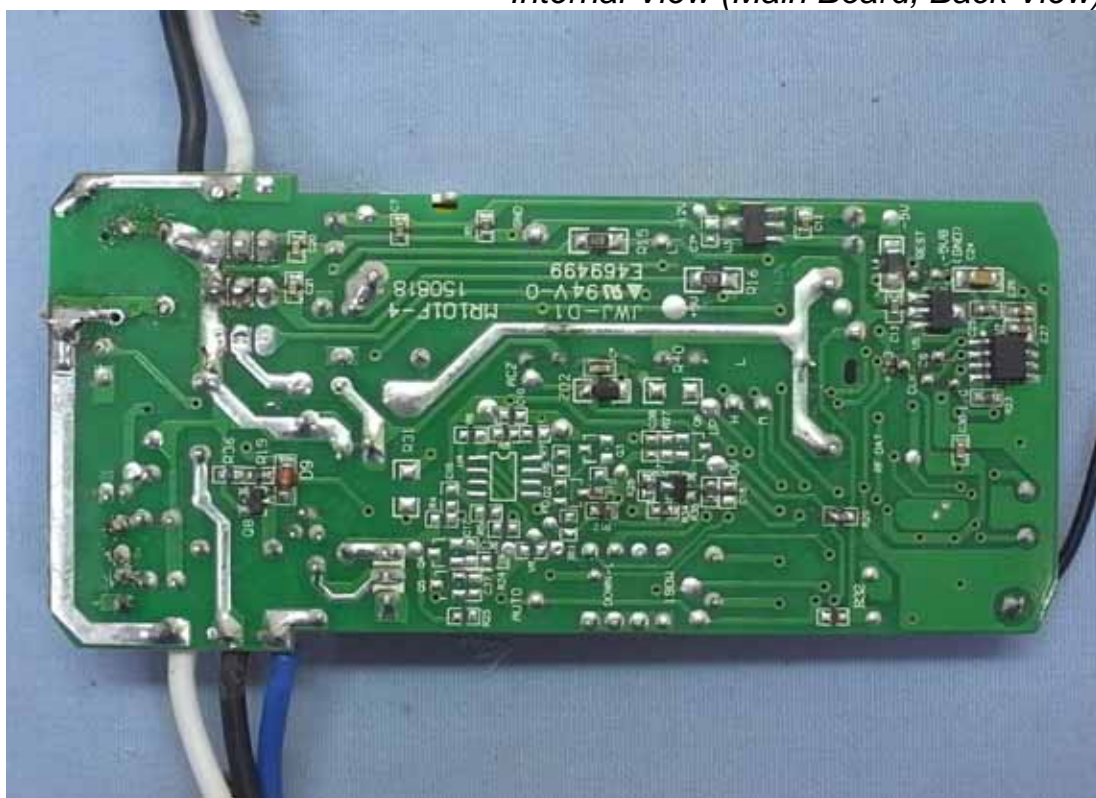
Figure 5 Internal View (Main Board, Back View)
