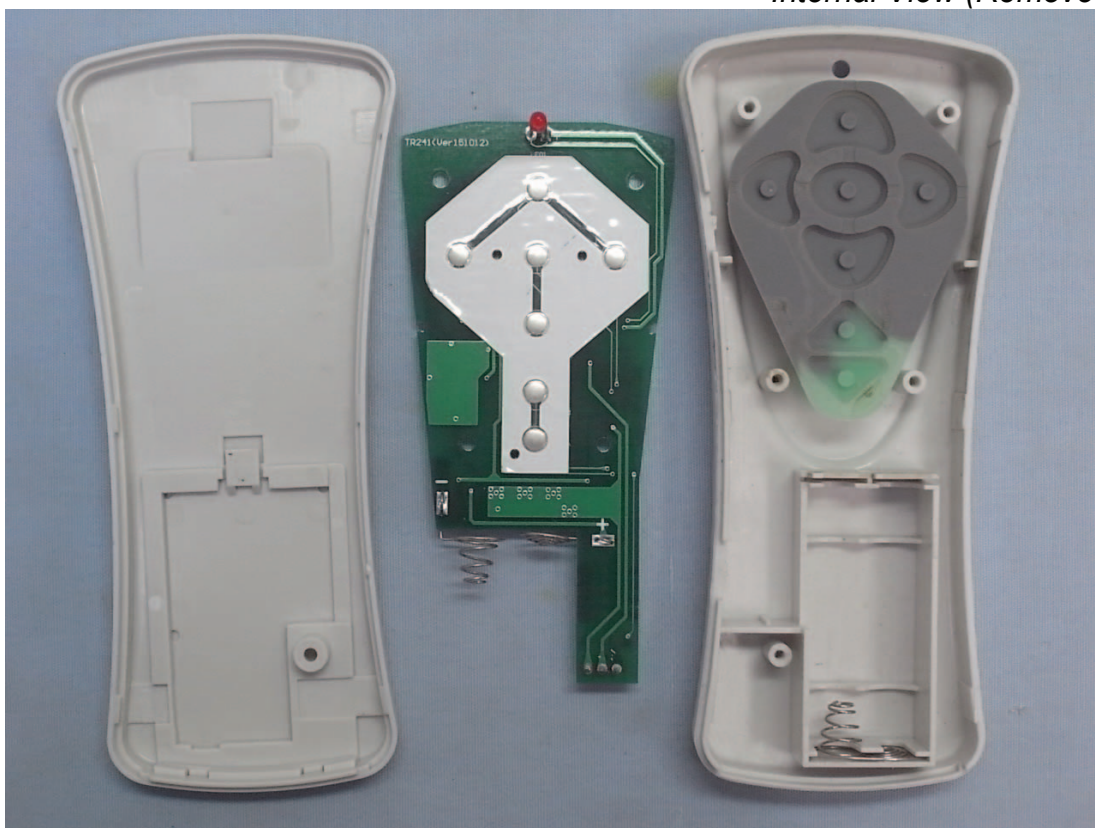
Photo 4 Internal View (Removed Cover)
