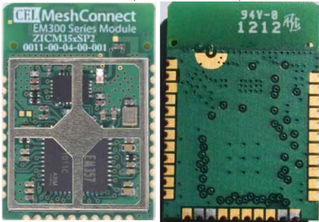
Figure 10 RF Module, Removed Shield Cover, Front & Back View
