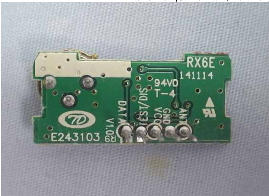
Figure 7 Internal View (Control Board, Front View)
