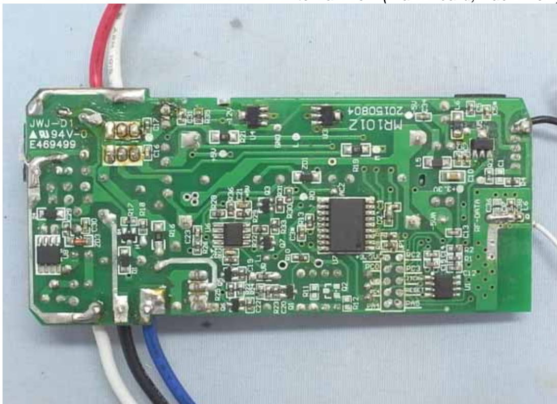
Figure 6 Internal View (Main Board, Back View)
