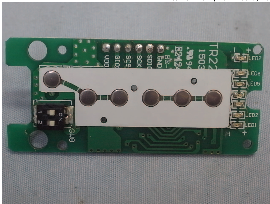
Photo 11 Internal View (Main Board, Back View)
