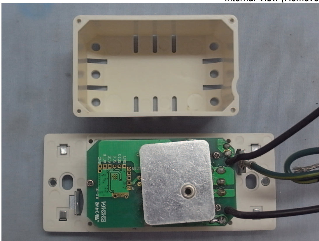
Photo 6 Internal View (Removed Cover)
