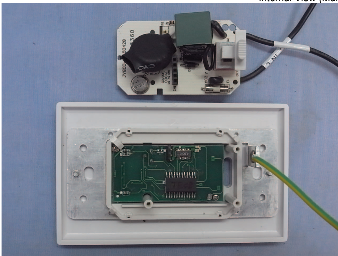
Photo 4 Internal View (Main Board)
