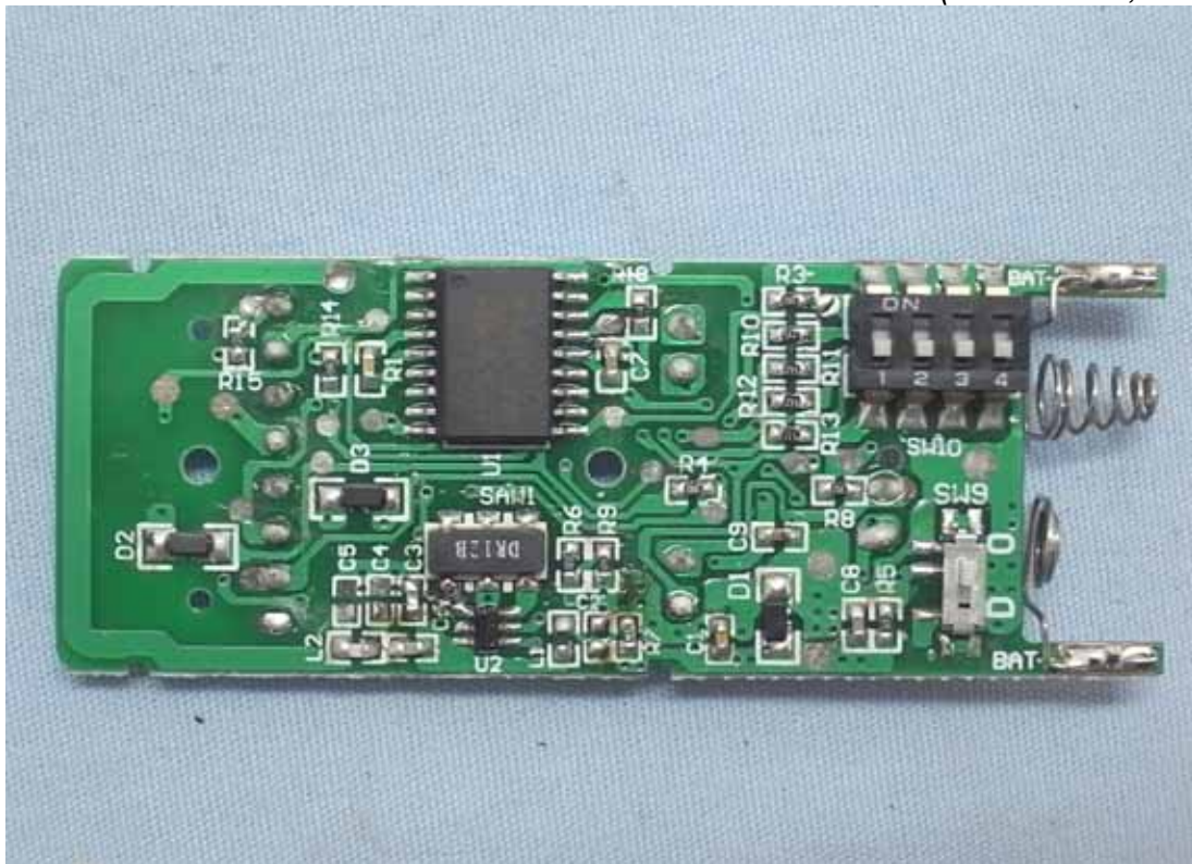
Photo 6 Internal View (Main Board, Front View)
