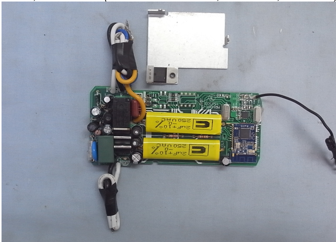
Figure 11 M/N: MR101F-3B, Internal View (Removed Shield Cover, Main Board, Front View)
