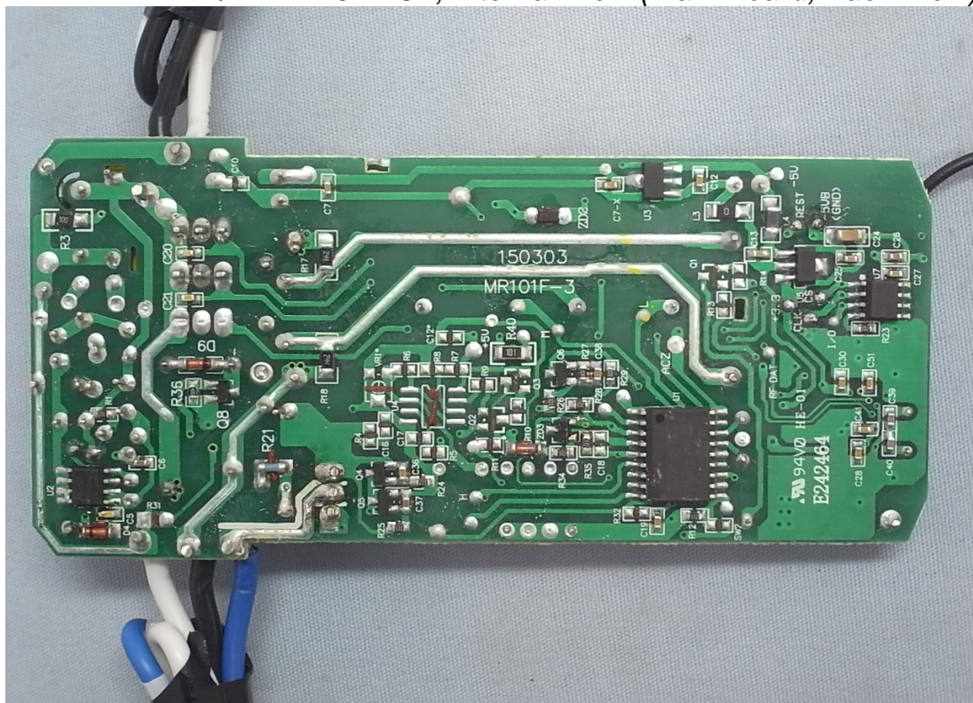
Figure 8 M/N: MR101F-3A, Internal View (Main Board, Back View)
