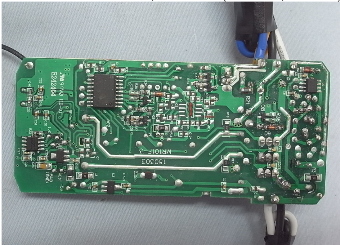
Figure 12 M/N: MR101F-3B, Internal View (Main Board, Back View)
