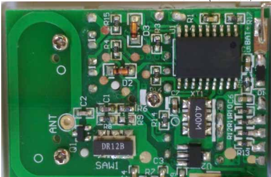
Photo 6 Internal View (Main Board, Front View)
