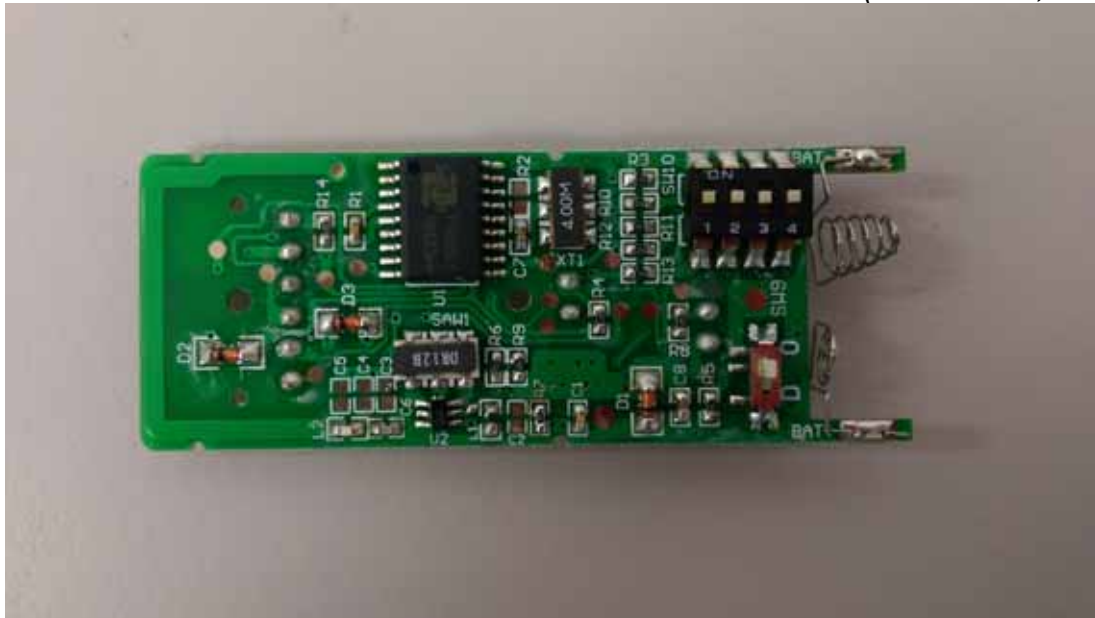
Photo 6 Internal View (Main Board, Front View)
