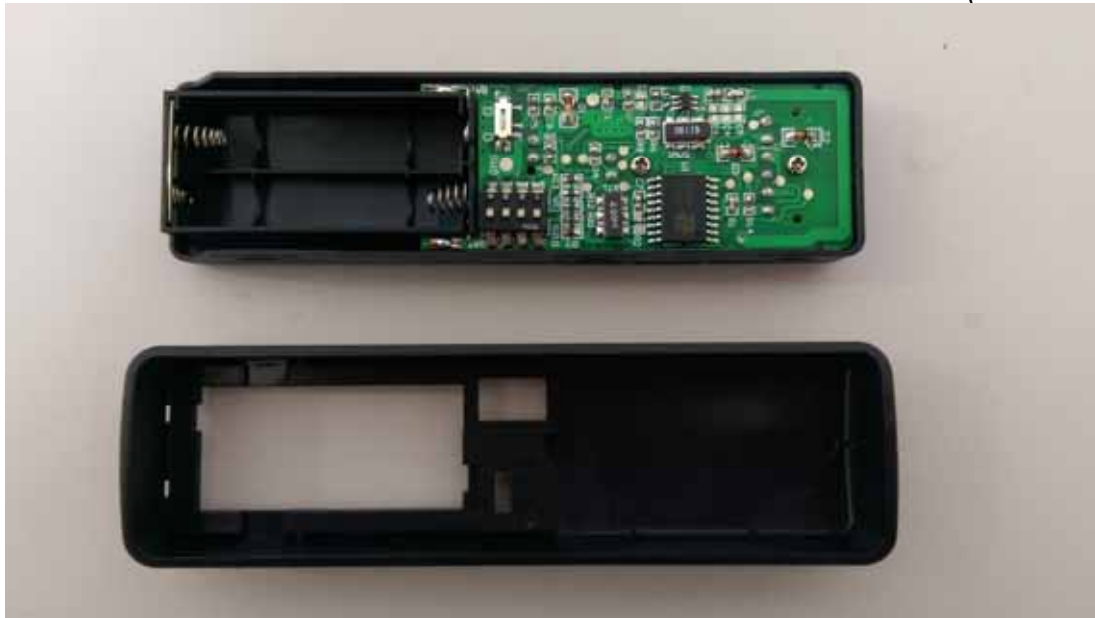
Photo 4 Internal View (Removed Cover)
