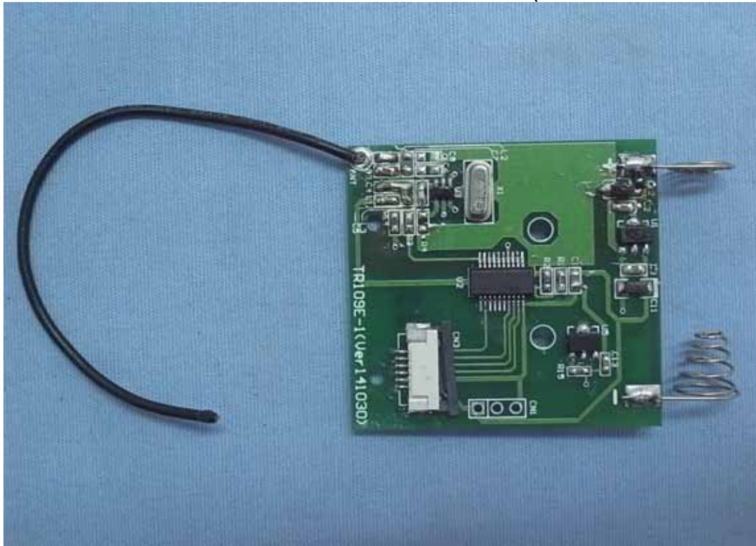
Photo 9 Internal View (RF Module Board, Front View)
