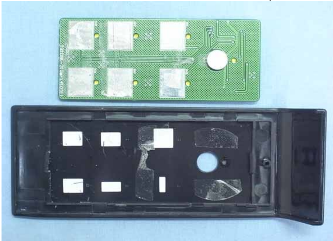
Photo 6 Internal View (Removed RF Module Board)
