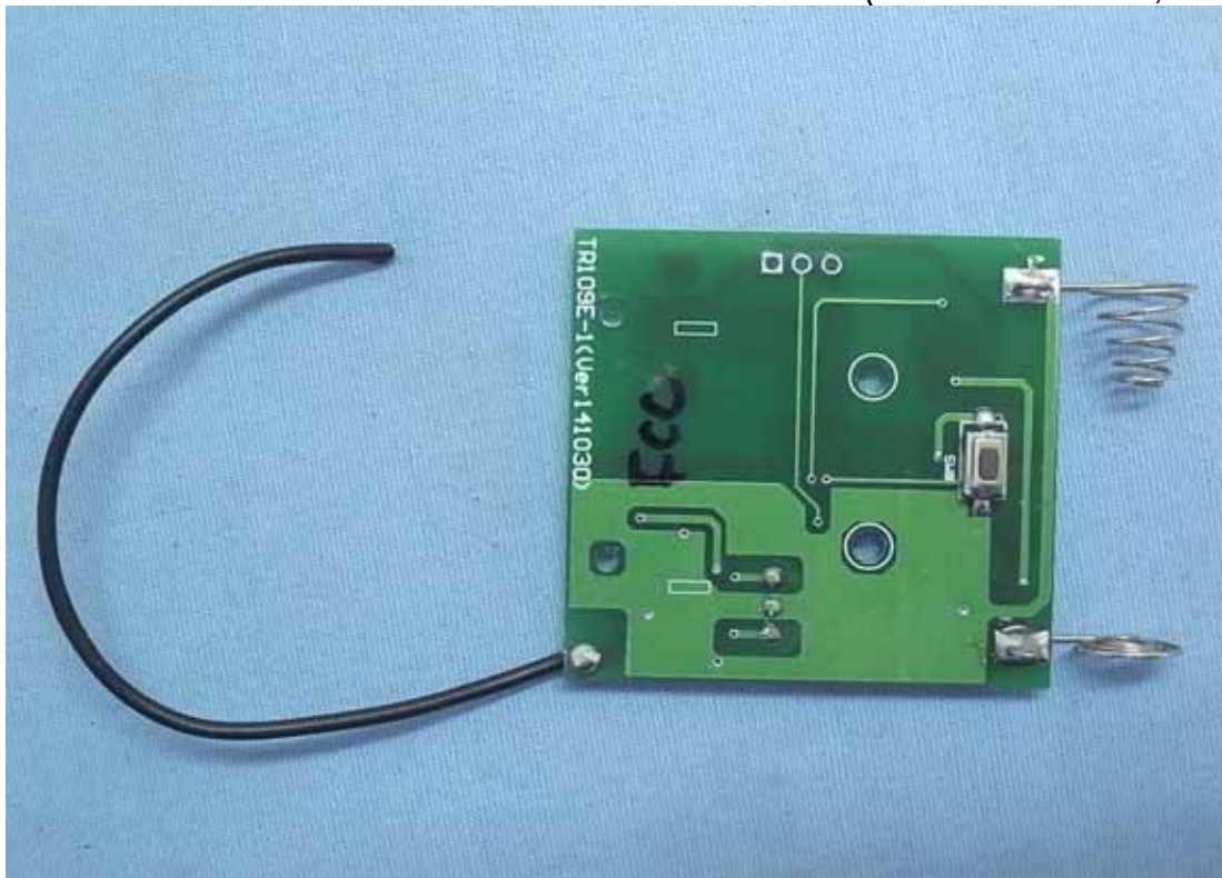
Photo 10 Internal View (RF Module Board, Back View)
