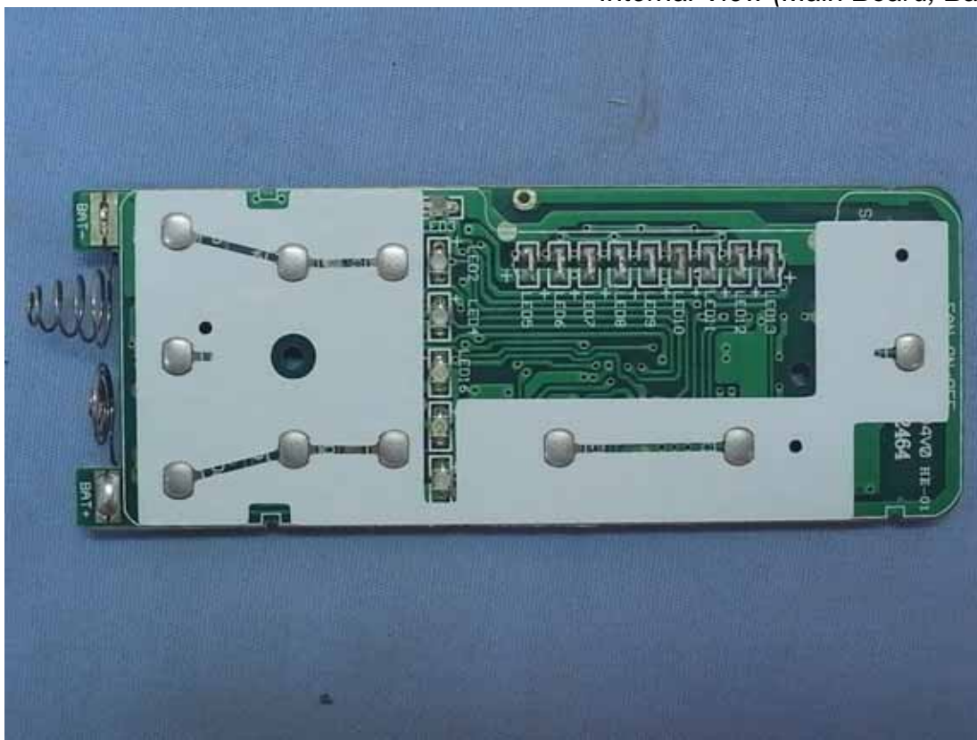
Photo 5 Internal View (Main Board, Back View)
