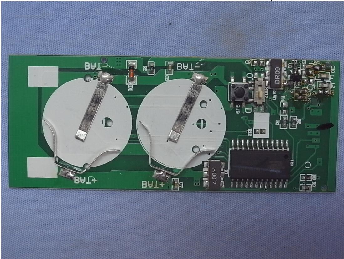
Photo 8 Internal View (Main Board, Front View)
