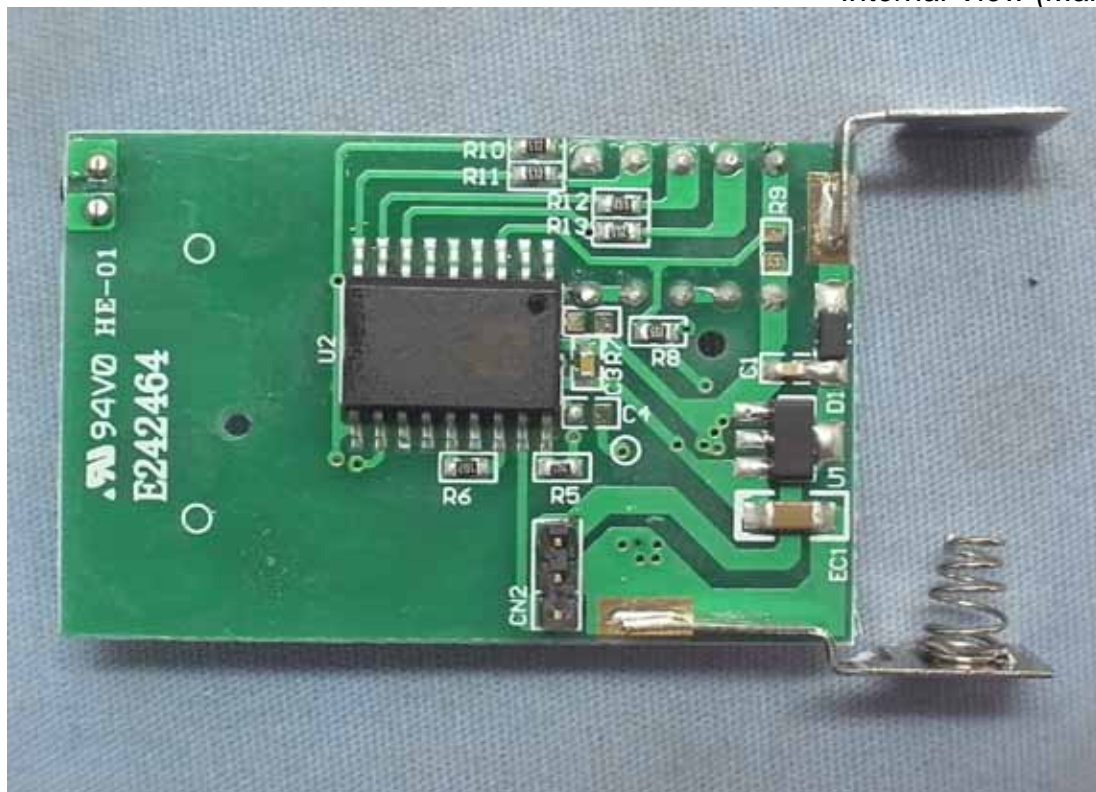
Photo 8 Internal View (Main Board)
