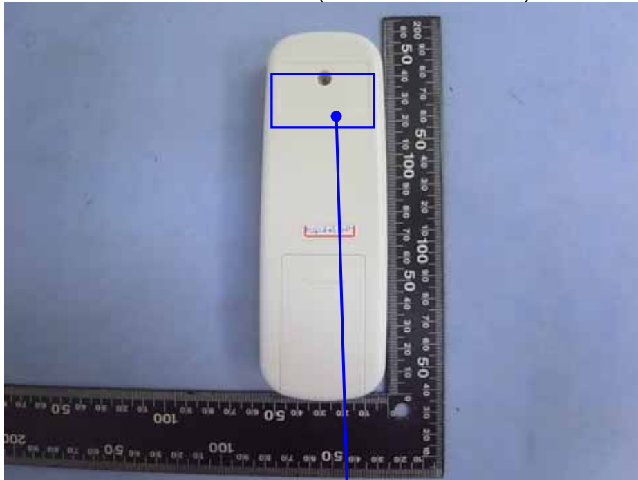
FCC ID/IC Label Placement
